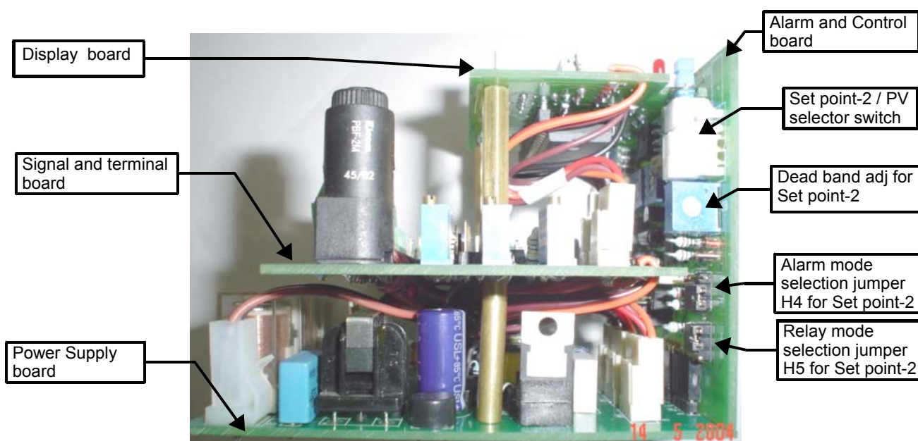
Fig-7: Instrument right side view
