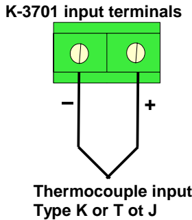
Fig-2: Input terminal arrangement
