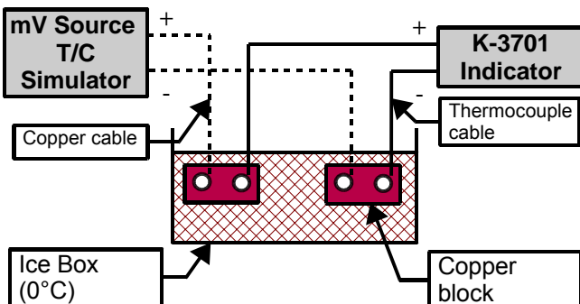
Fig-3: Connection drawing
