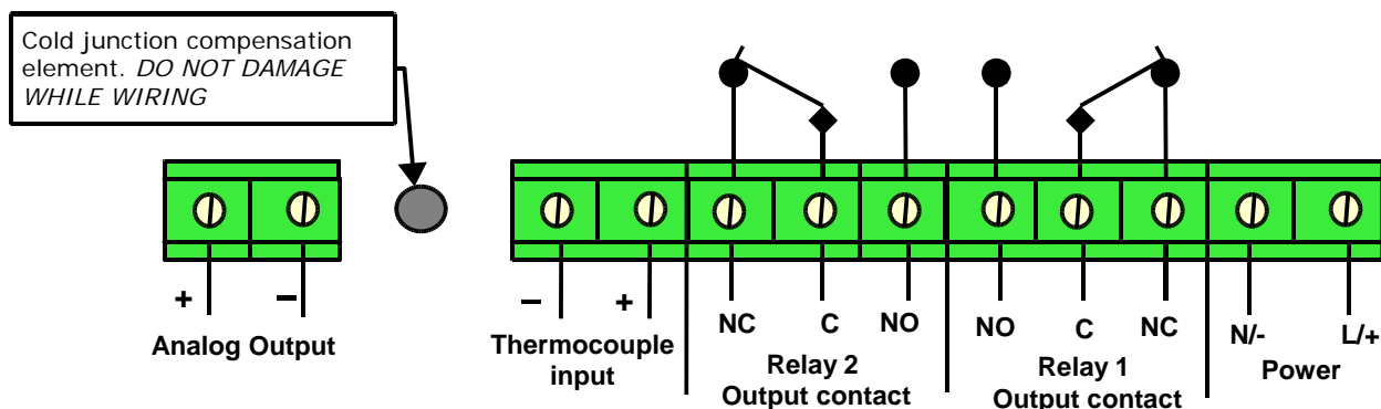
Fig-6: Instrument top view
