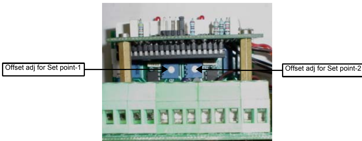
Fig-9: Alarm and control for Offset pot location
